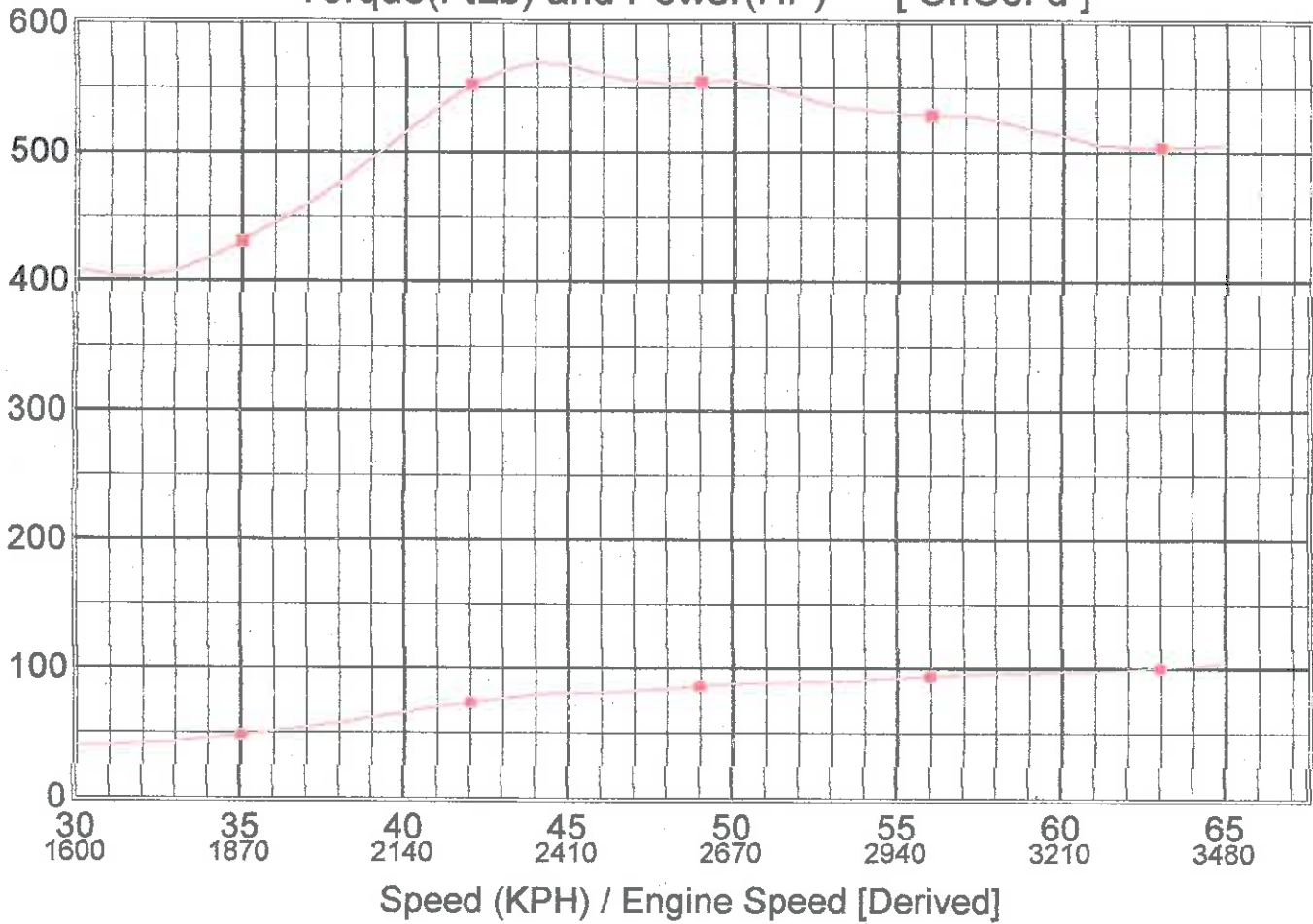
Torque(FtLb) and Power(HP) [ UnCor'd ]
